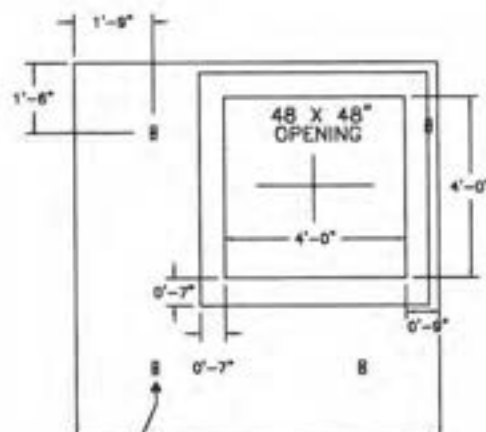
PLAN VIEW FOR COVER
