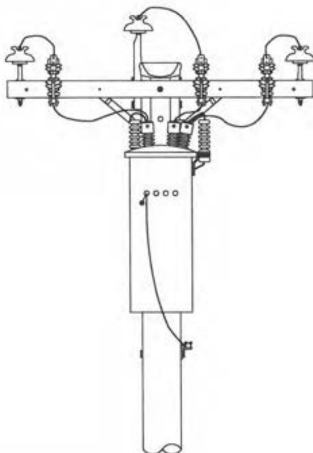
FRONT VIEW
