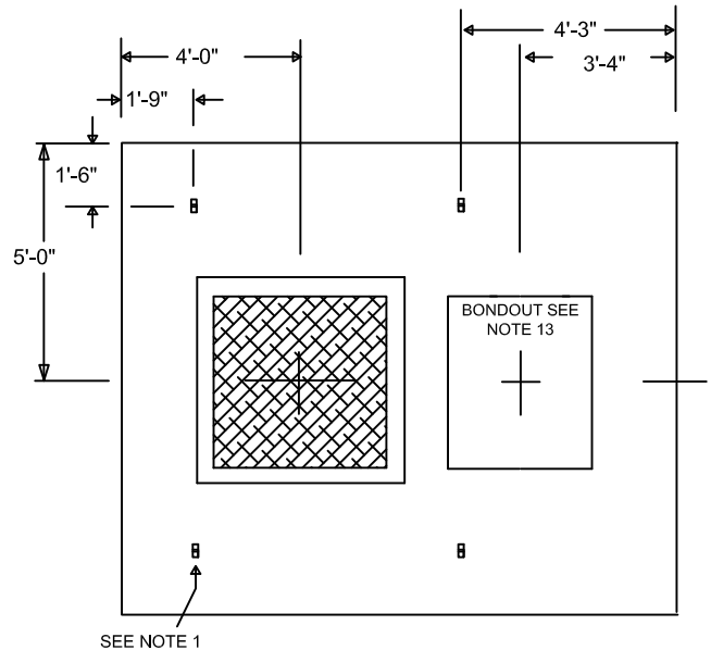
PLAN VIEW FOR COVER
