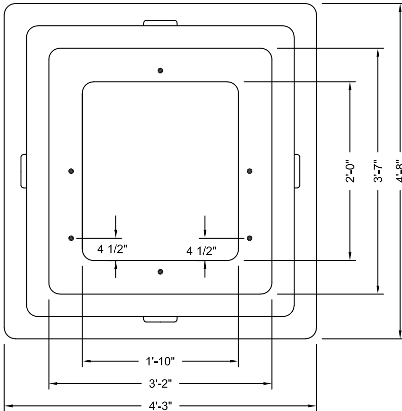
PLAN VIEW
